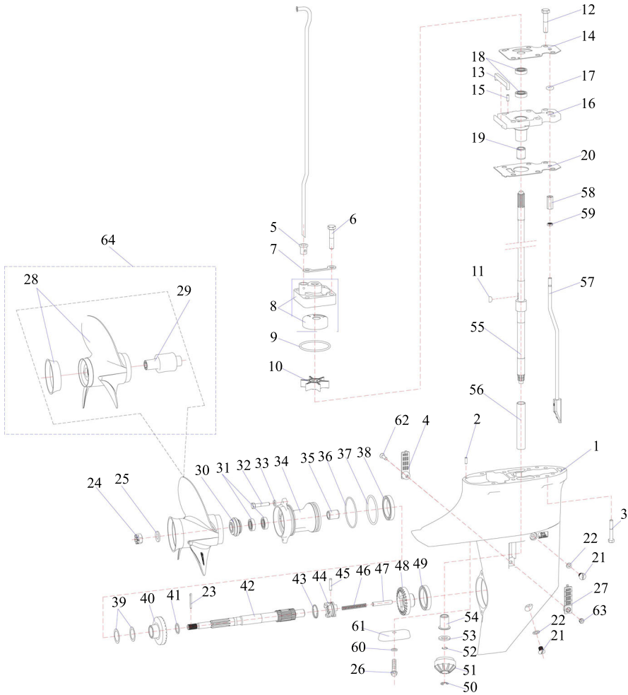
Lower units
