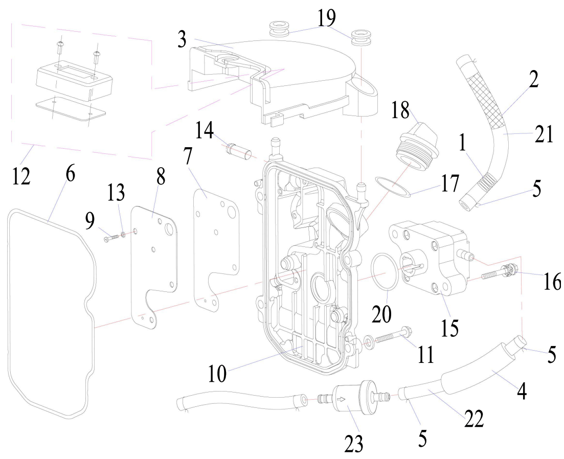
Cylinder Head Assy.
