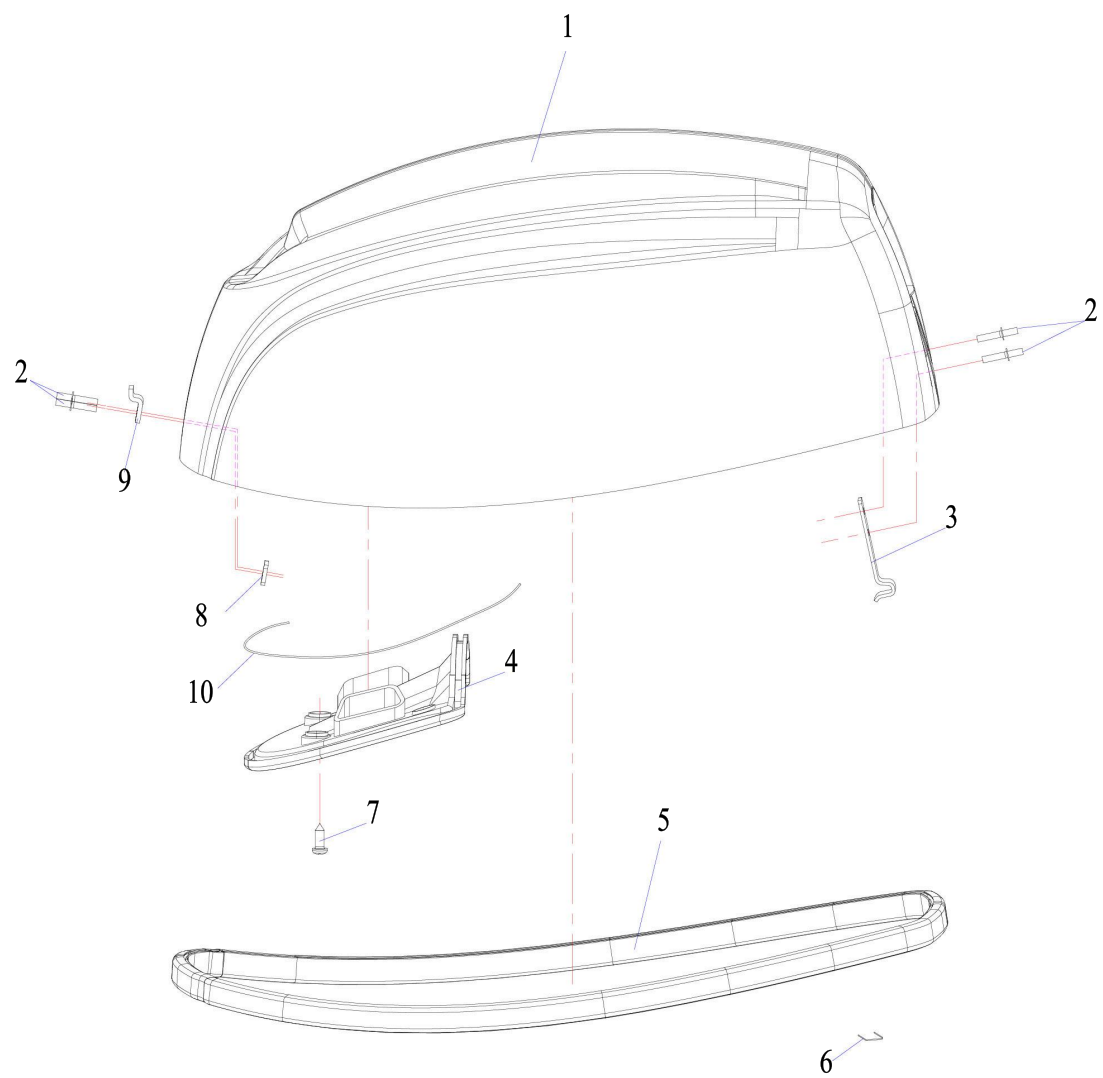
Top cowling
