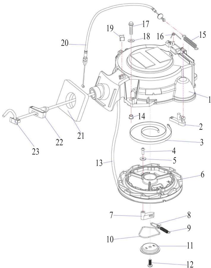
Starter Cover Assy.
