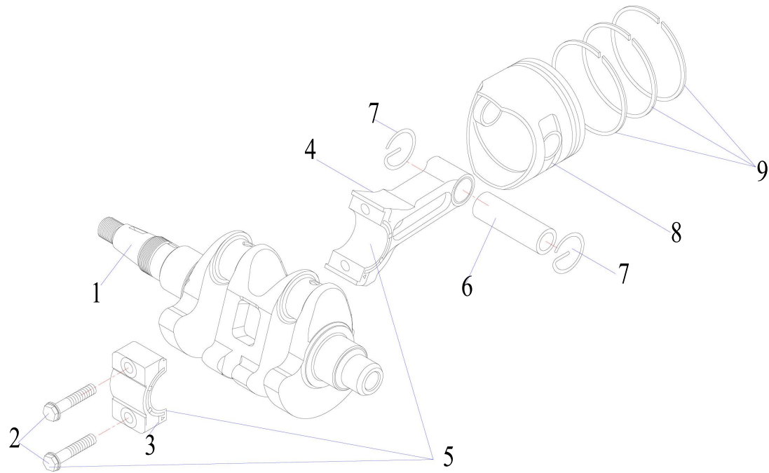
Crank & Rod Assy.
