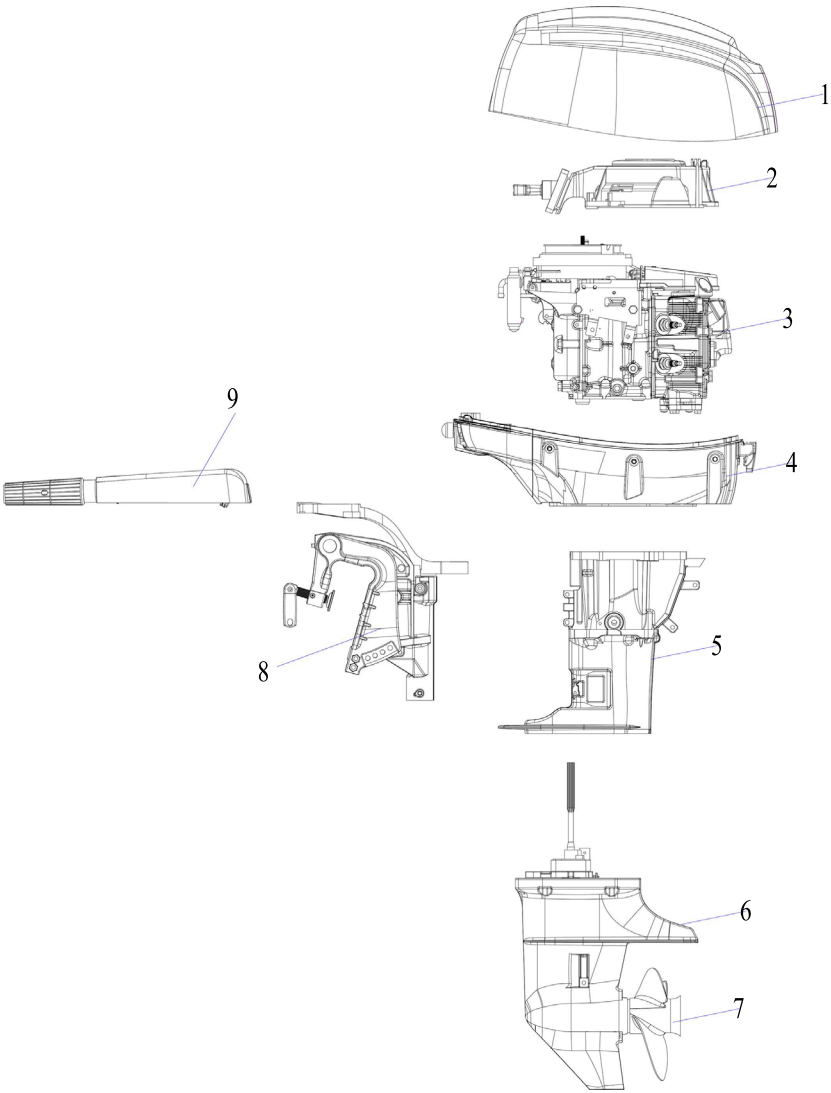
General Assy
